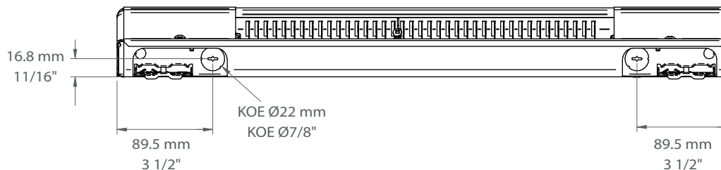
Bottom View
